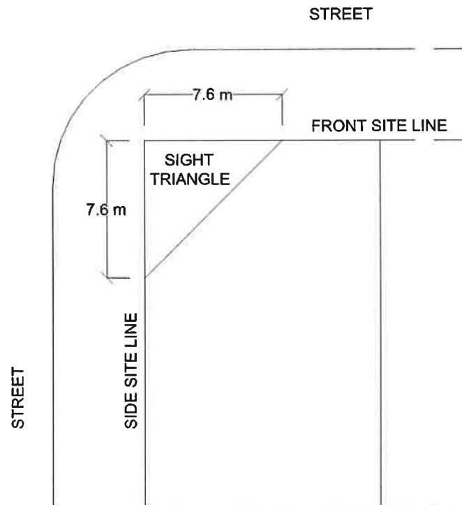
Figure 2-2: Sight Triangle
